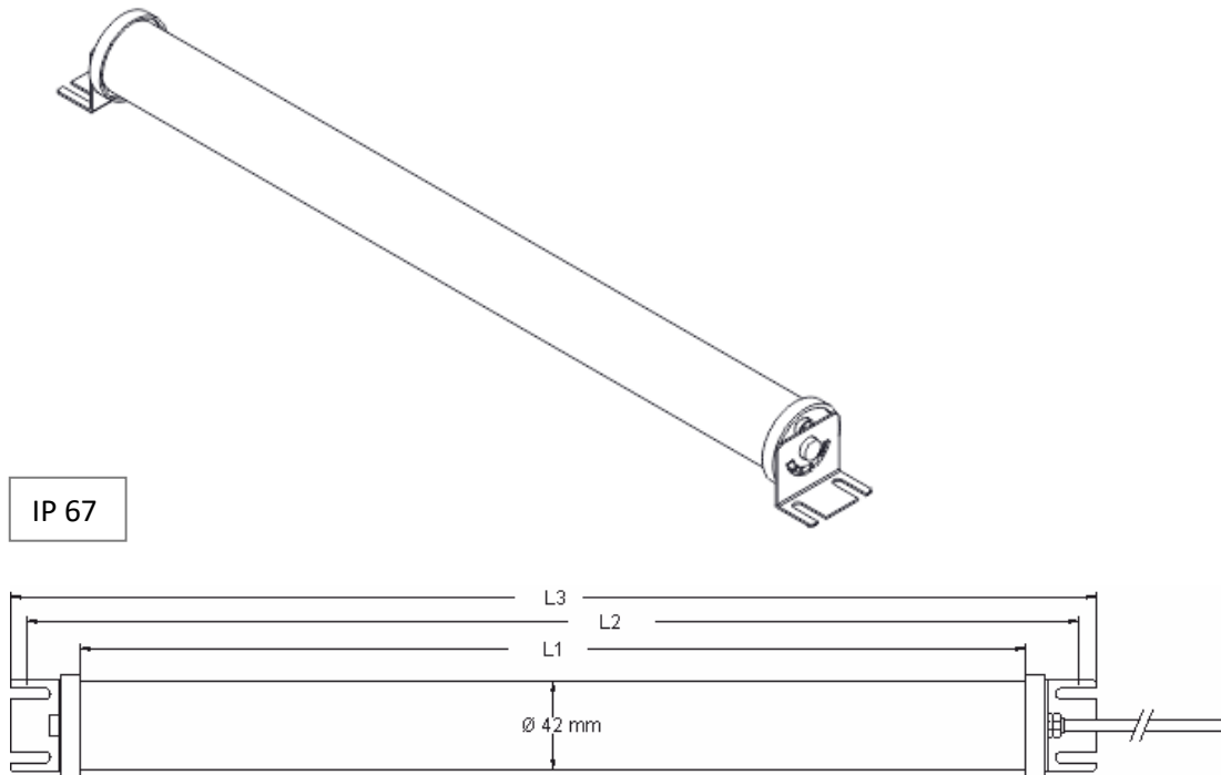
Product Dimension Drawing All dimensions in mm
