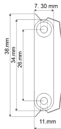
Installation Dimension
