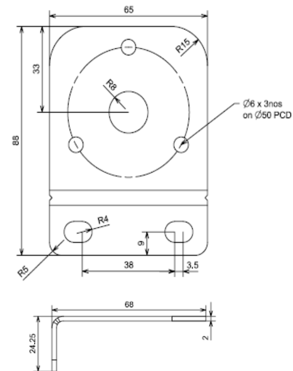
SIDE VIEW BEND PROFILE
