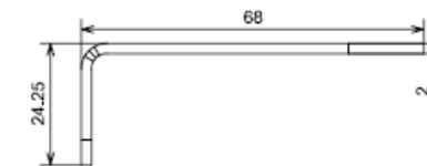
SIDE VIEW BEND PROFILE
